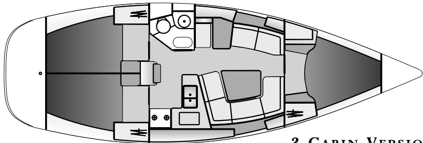
3 CABIN VERSION
