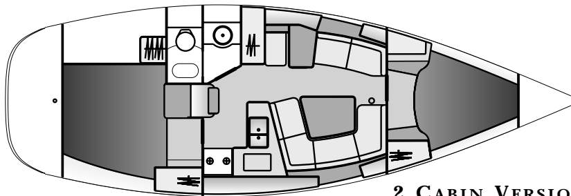
2 CABIN VERSION
